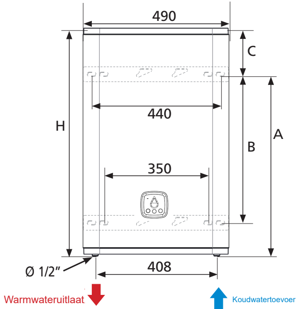
Verticale wandboiler
